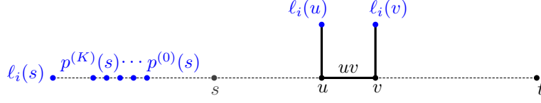
■ Figure 2 Worst-case stretch when triangulating via portal p^0(s) . There are K + 1 portals closer than \ell_i(s) . When computing distances from/to these portals, the edges of the (1, 6) -spanner were used, hence the distortion is bounded.
